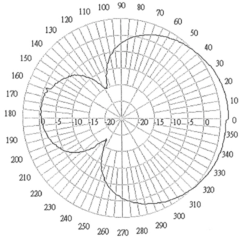
A-133 GPS Active Antenna RHCP response / ANTENNA RADIATION PATTERN
